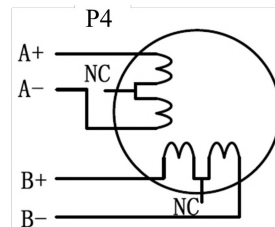
Figure 9 6-lead motor full coil connection
