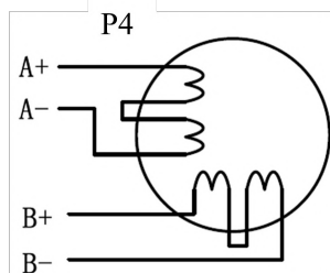
Figure 10 8-lead motor series connection
