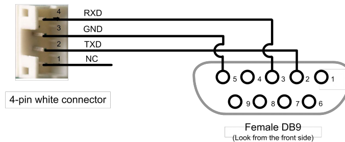
Figure 3: RS232 connector
