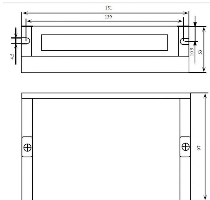
Figure 1 Mechanical specifications
