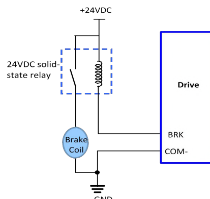
Figure 8 Brake output
